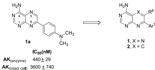
Figure 1. Adenosine kinase inhibitor high-throughput screening hit 1a , and novel pyridopyrimidine AK inhibitor 2 .
