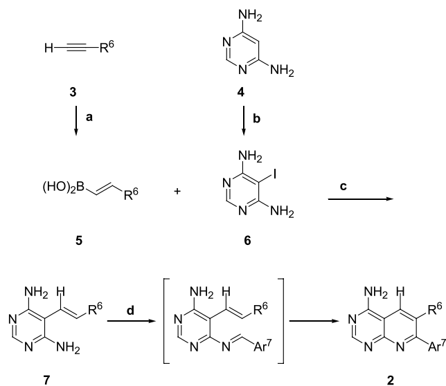
Scheme 1. Reagents and conditions: (a) catecholborane, THF, reflux, 100%; (b) I_2 , K_2CO_3 , DMF/H 2 O, 45 °C, 65%; (c) (PPh_3)_4Pd , (aq) Na_2CO_3 , THF, reflux, 50–80%; (d) Ar^7CHO , 1,2,4-trichlorobenzene or diphenyl ether, 215–260 °C, air, 15–25%.
